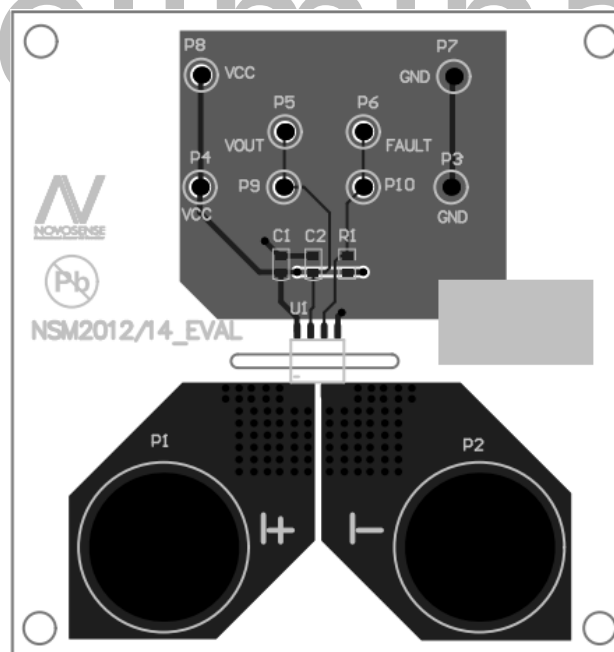
Figure 6.2 NSM2016 PCB Layout
