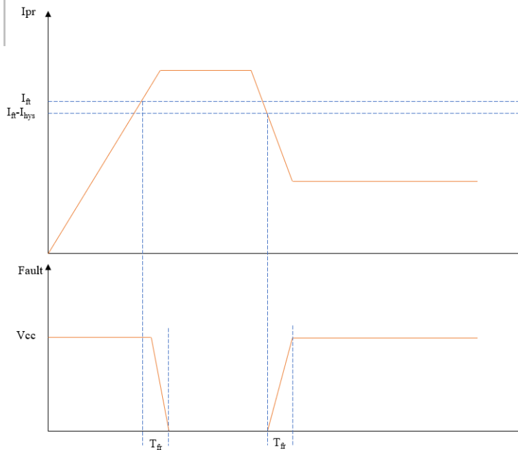
Figure 5.1 NSM2016 过流表现
