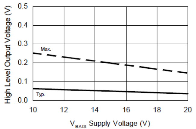
Figure 14B. High Level Output vs. Supply Voltage
